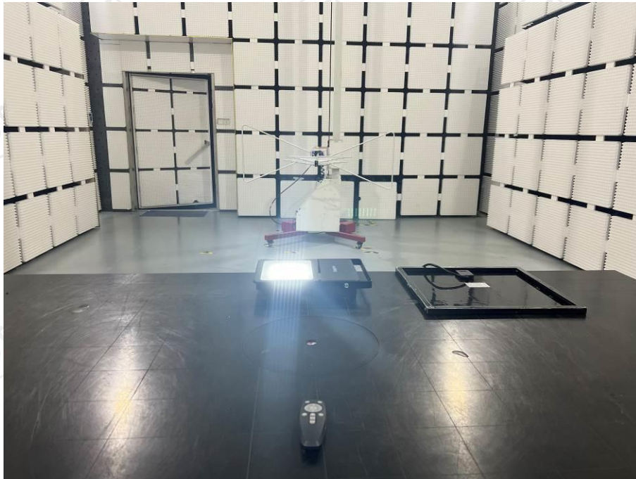
Radiated electromagnetic disturbances (30 MHz to 1 GHz) test view
